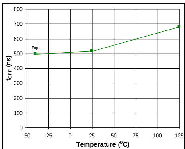
Fig. 10. (Toff_Hs21) Turn-off Propagation Delay vs. Temperature
