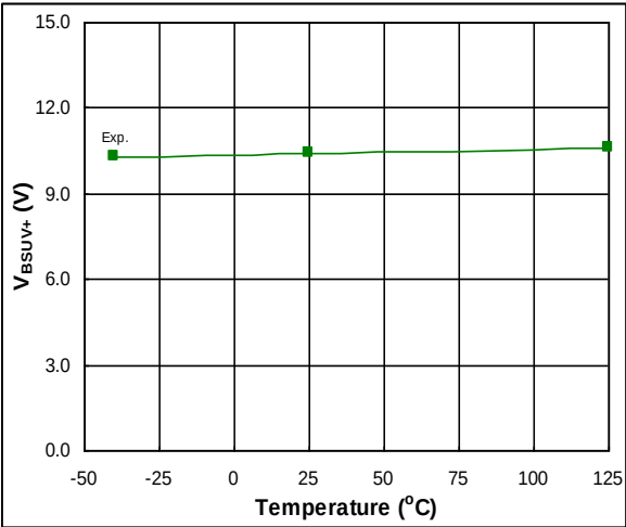
Fig. 36. V_{BS} Supply Undervoltage Positive Going Threshold vs. Temperature
