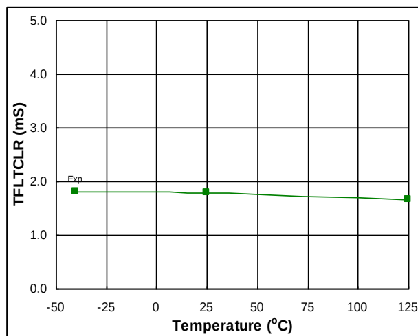
Fig. 20. FAULT Clear Time vs. Temperature
