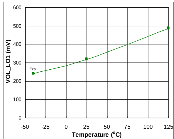
Fig. 25. Low Level Output Voltage vs. Temperature
