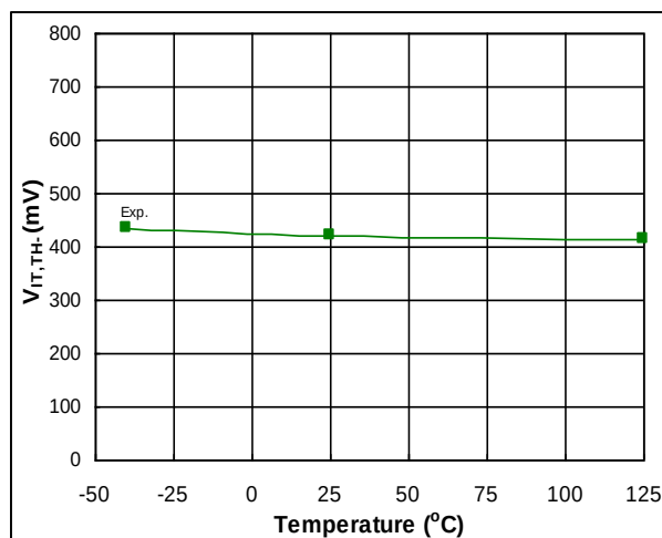
Fig. 24. ITRIP Input Negative Going Threshold vs. Temperature
