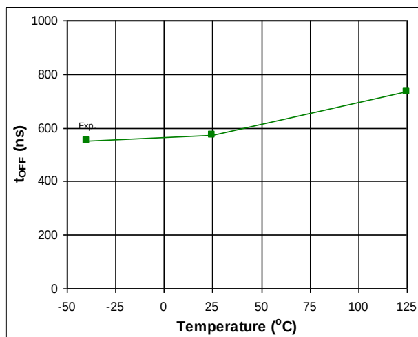
Fig. 8. (Toff_Ls1) Turn-off Propagation Delay vs. Temperature
