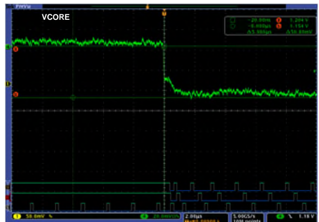
Figure 35: Phase Add 1Φ→3Φ
