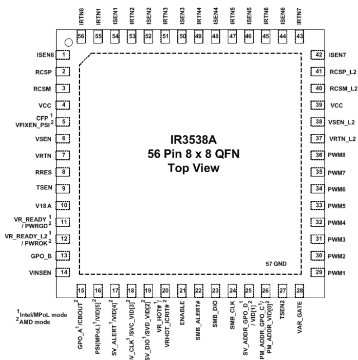
Figure 4: IR3538A Package Top View, Enlarged
