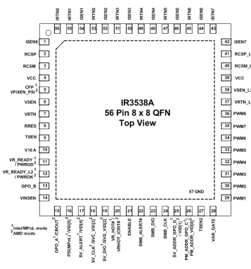
Figure 2: IR3538A Package Top View
