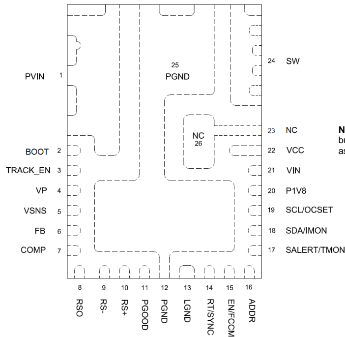
Figure 3: IR38062 package (Top View) 5mm x 7mm PQFN
