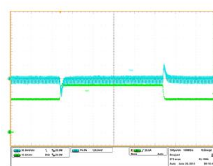
Figure 50: Transient Response, 24.5A to 35A step (2.5A/us)
