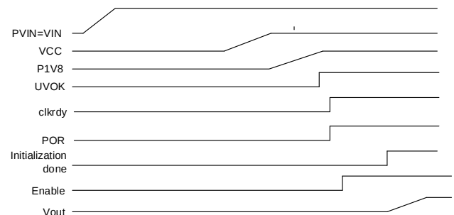
Figure 11: IR38064 Initialization sequence
