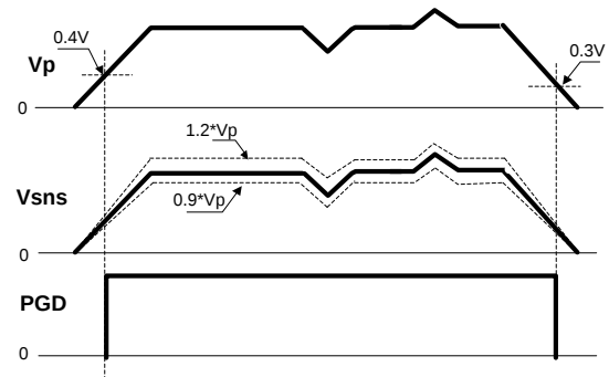
Figure 30: V_p Tracking ( \text{Track\_En} = 0V )
