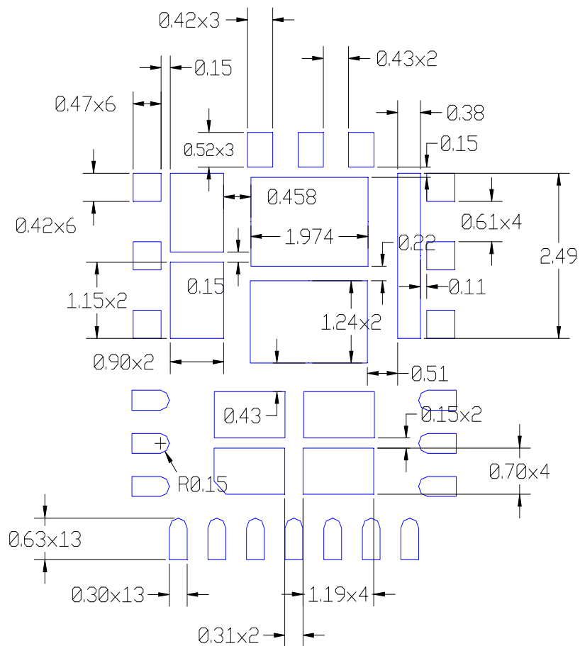
Stencil Aperture All Dimensions in mm
