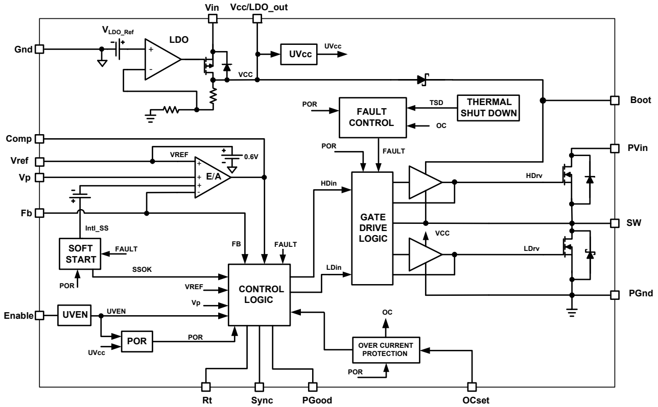
Fig. 2. Simplified block diagram of the IR3837
