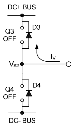
Figure 17: D3 conducting
