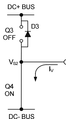
Figure 18: Q4 conducting
