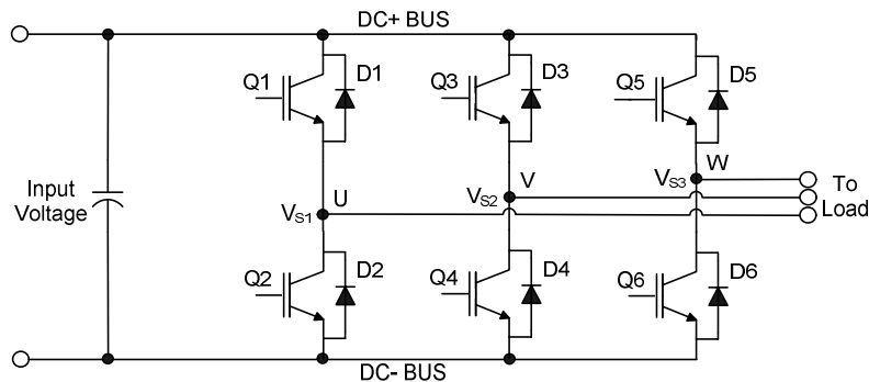
Figure 14: Three phase inverter
