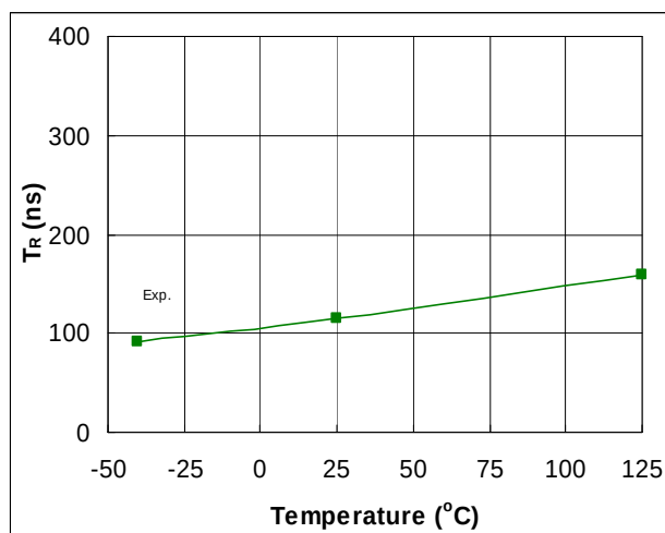
Fig. 29. Turn-on Rise Time vs. Temperature
