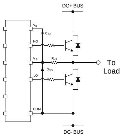
Figure 26: V_S clamping diode
