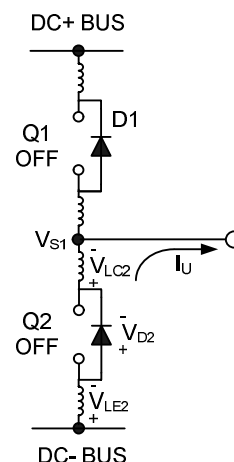
Figure 21: V_S negative
