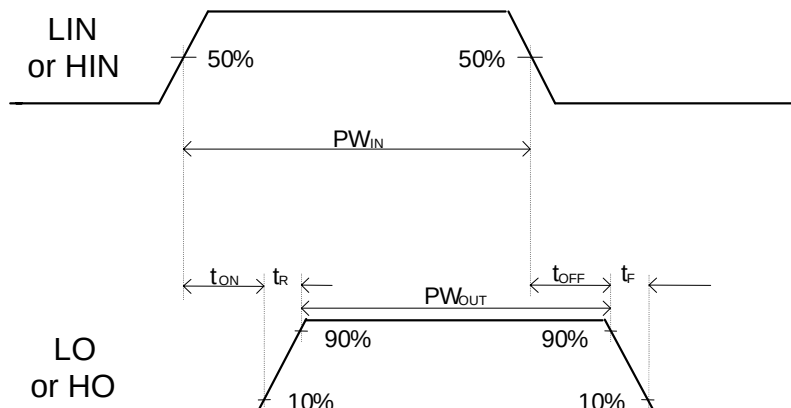
Figure 3: Switching time waveforms
