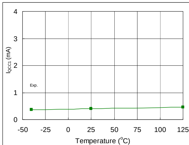
Fig. 34. Quiescent VCC Supply Current vs. Temperature
