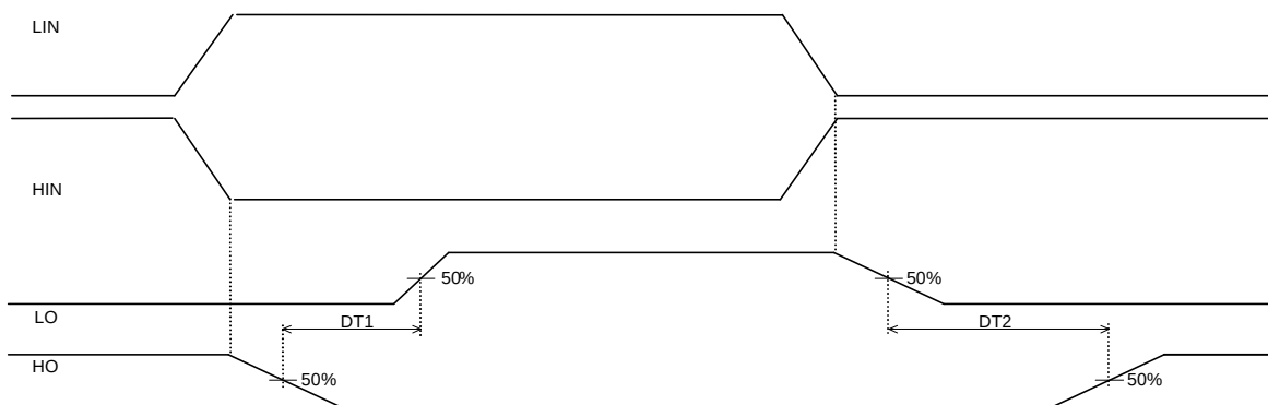
Figure 5: Deadtime definition
