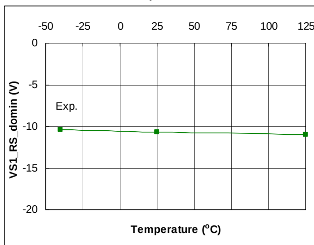
Fig. 44. Max -Vs vs. Temperature
