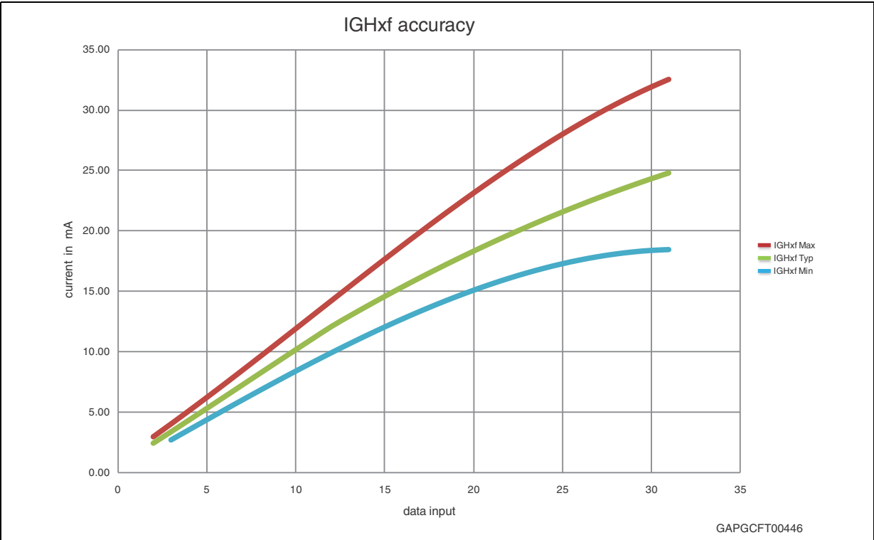
Figure 7. IGHxf ranges
