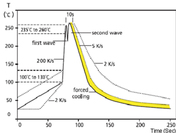
建議 double-wave Soldering Profile
