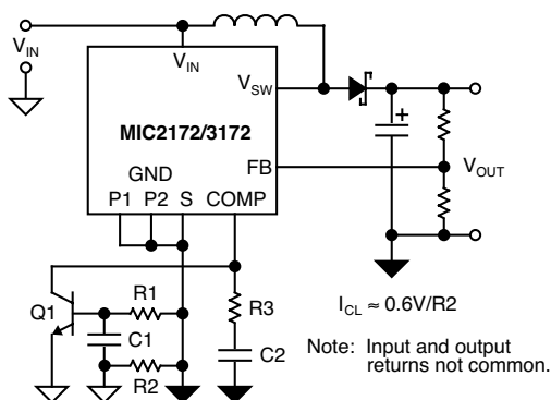
Figure 9. Current Limit
