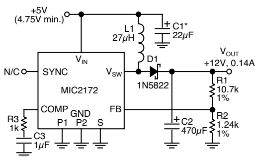
Figure 1. MIC2172 5V to 12V Boost Converter
