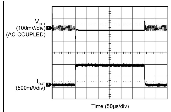
FIGURE 2-28: Load Transient (50 mA to 1A).
