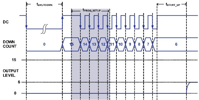
Figure 12. Presetting Timing
