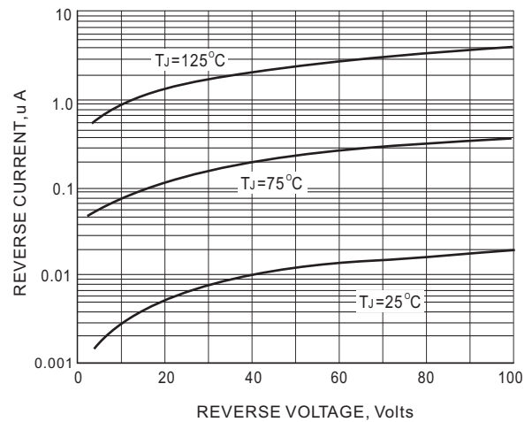
FIG. 2-TYPICAL REVERSE CHARACTERISTICS
