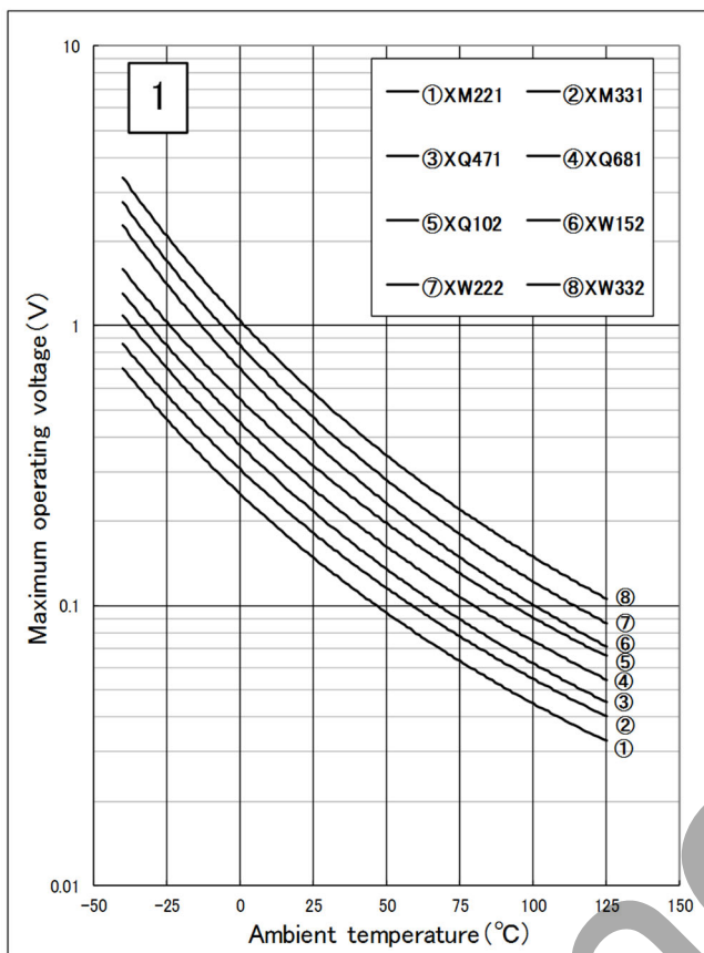
Graph of Maximum Operating Voltage Reduction Characteristics
