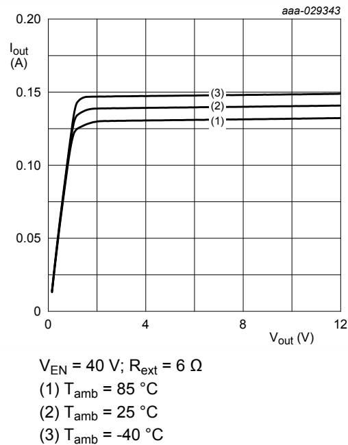
Fig. 8. NCR420U: Output current as a function of output voltage; typical values
