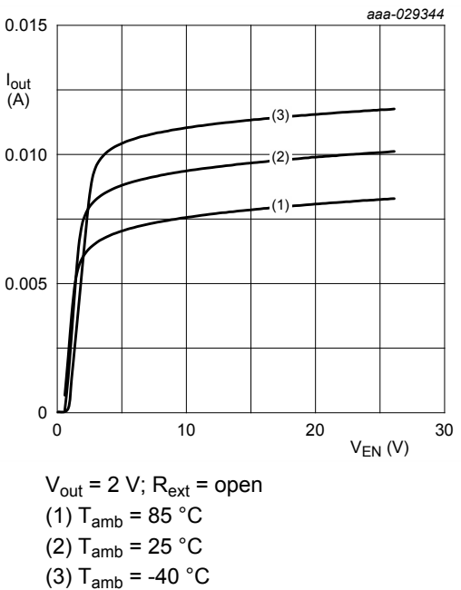
Fig. 9. NCR420U: Output current as a function of enable voltage; typical values
