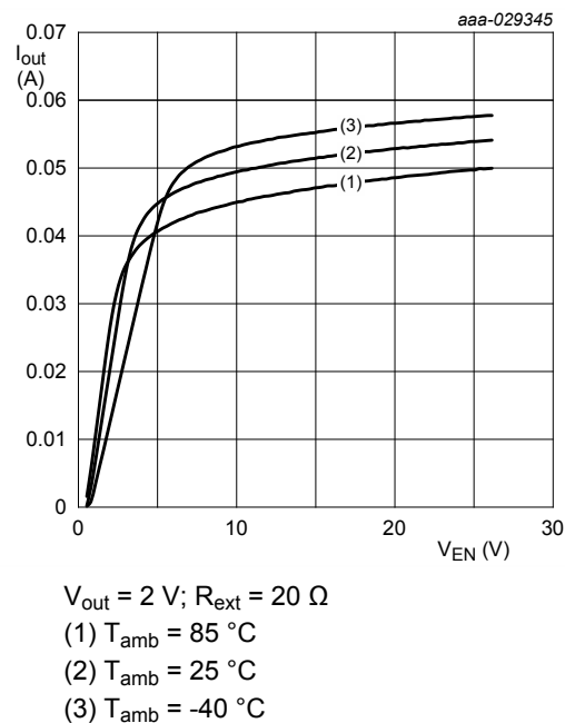
Fig. 10. NCR420U: Output current as a function of enable voltage; typical values
