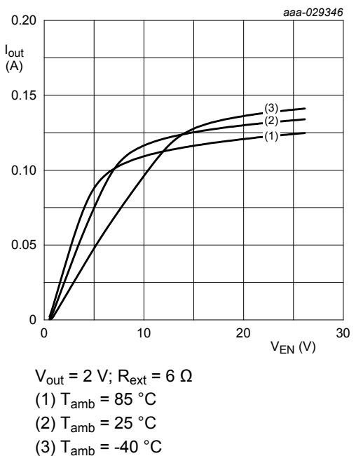
Fig. 11. NCR420U: Output current as a function of enable voltage; typical values
