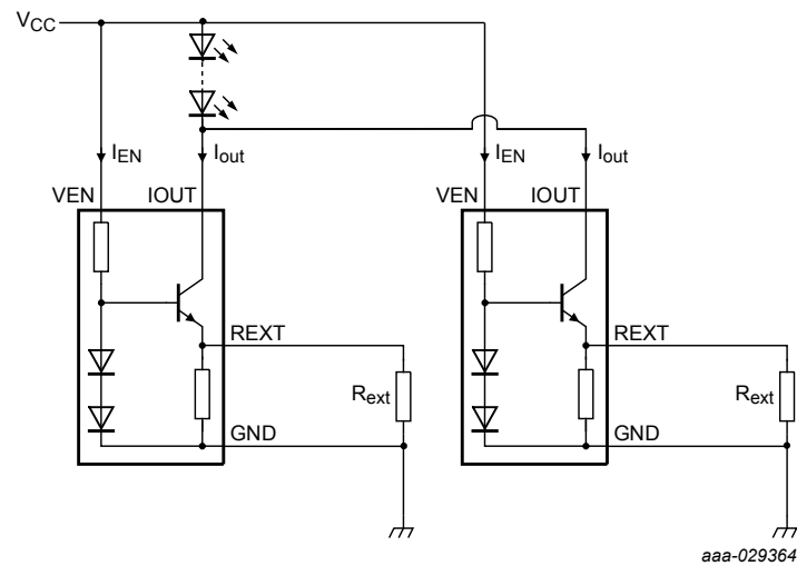
Fig. 26. Application diagram: Parallelization
