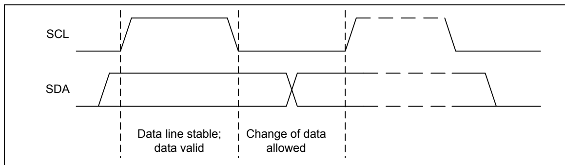
Figure 5-22 Bit Transfer on the I²C bus
