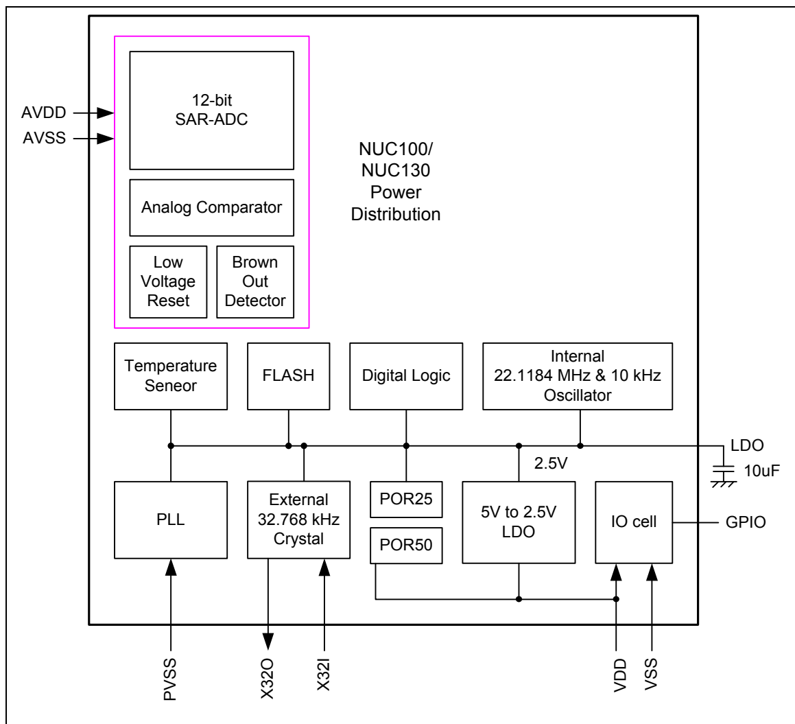
Figure 5-3 NuMicro™ NUC100/ NUC130 Power Distribution Diagram
