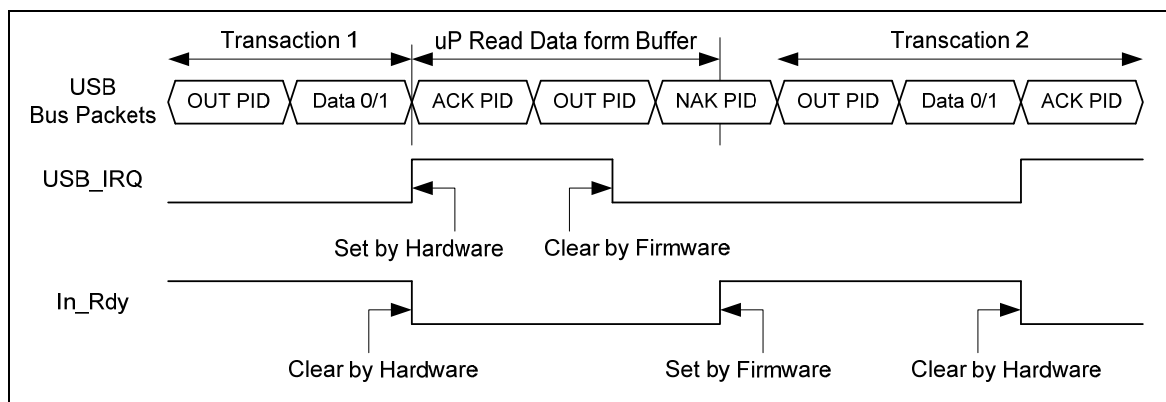
Figure 5-13 Data Out Transfer
