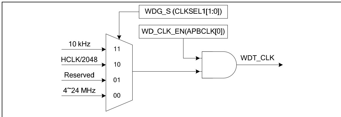
Figure 5-65 Watchdog Timer Clock Control
