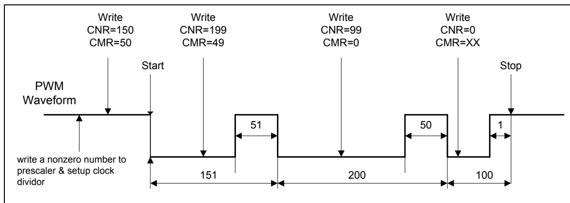
Figure 5-42 PWM Double Buffering Illustration
