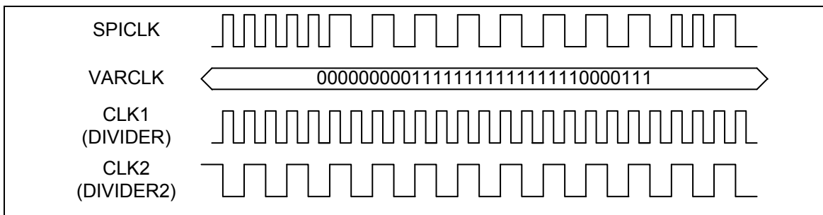
Figure 5-52 Variable Serial Clock Frequency
