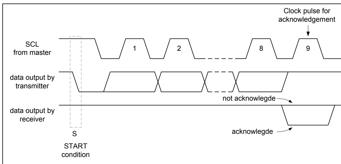
Figure 5-23 Acknowledge on the I²C bus
