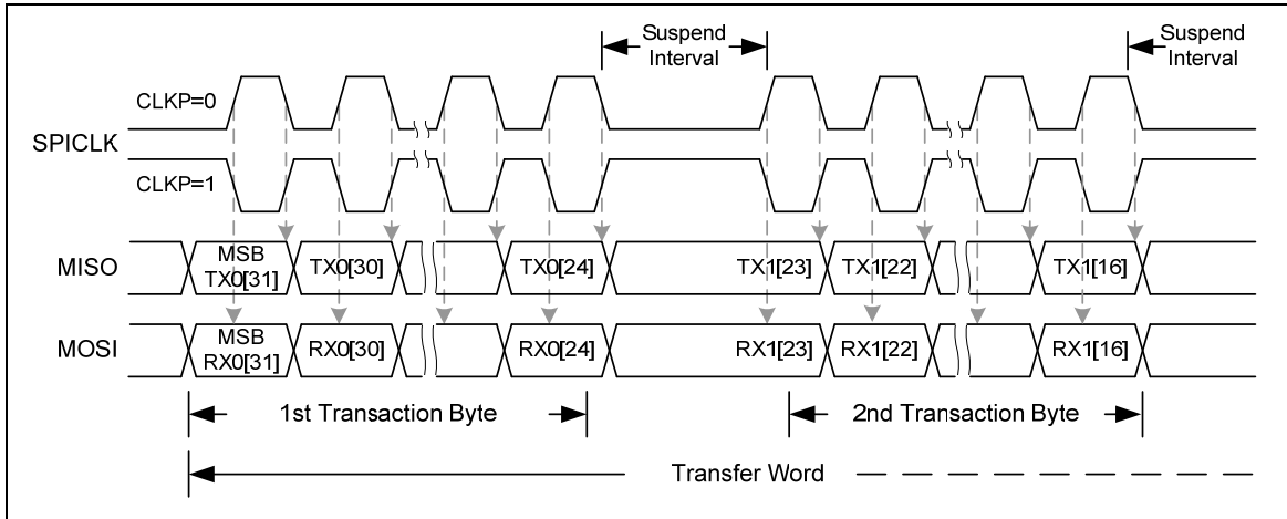
Figure 5-56 Timing Waveform for Byte Suspend
