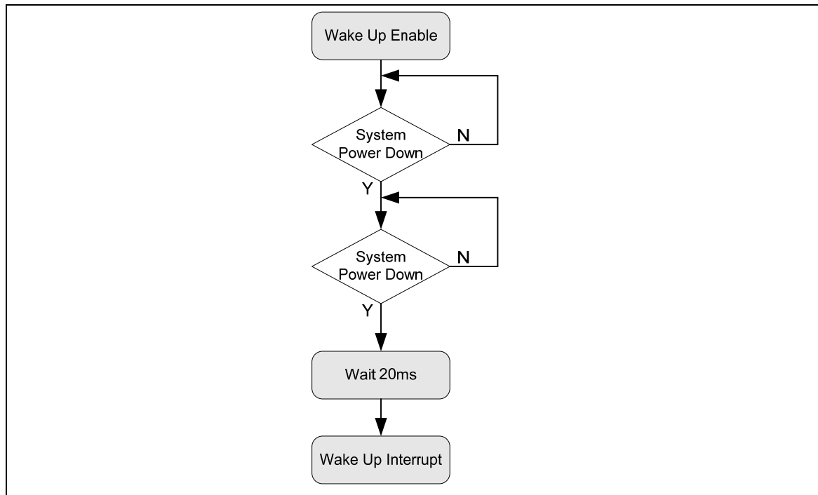
Figure 5-10 Wakeup Interrupt Operation Flow
