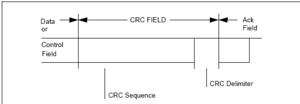
Figure 5-79 Format of CRC FIELD
