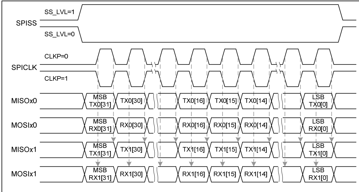
Figure 5-57 Two Bits Transfer Mode
