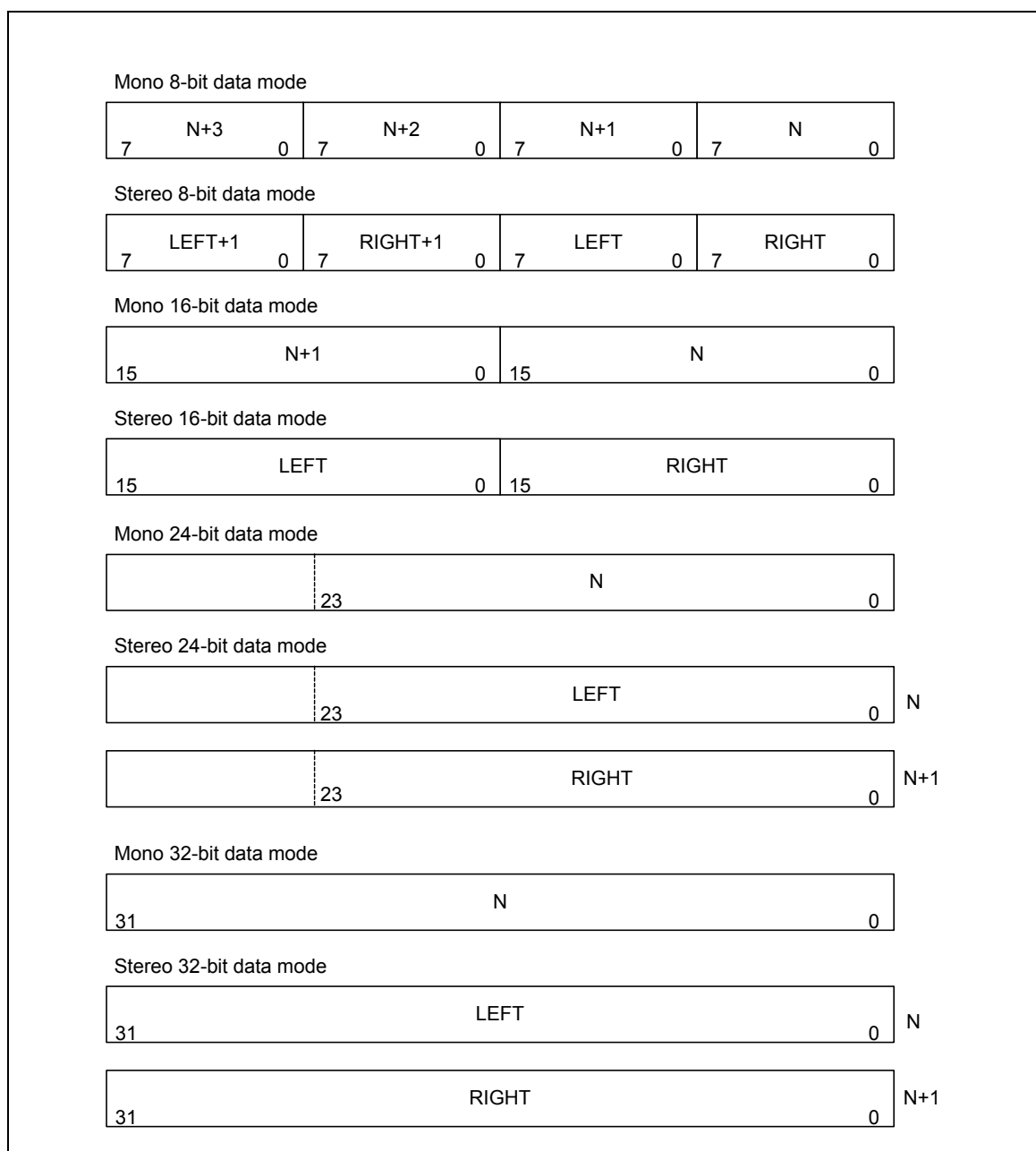
Figure 5-93 FIFO contents for various I 2 S modes
