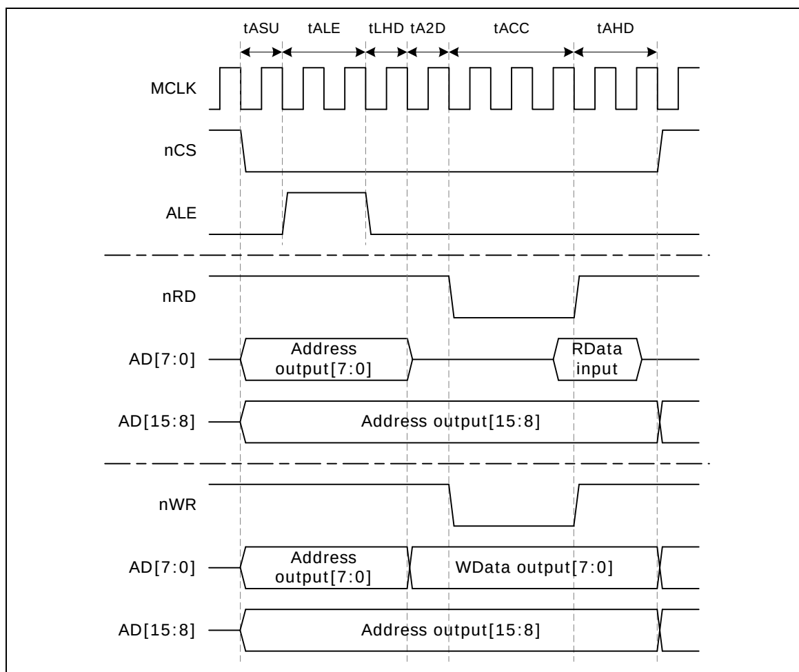
Figure 5-112 Timing Control Waveform for 8bit Data Width
