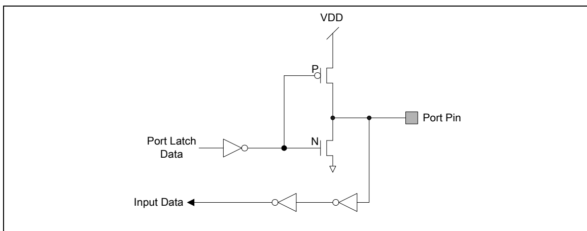
Figure 5-14 Push-Pull Output
