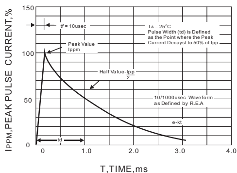
Fig.3 PULSE WAVEFORM
