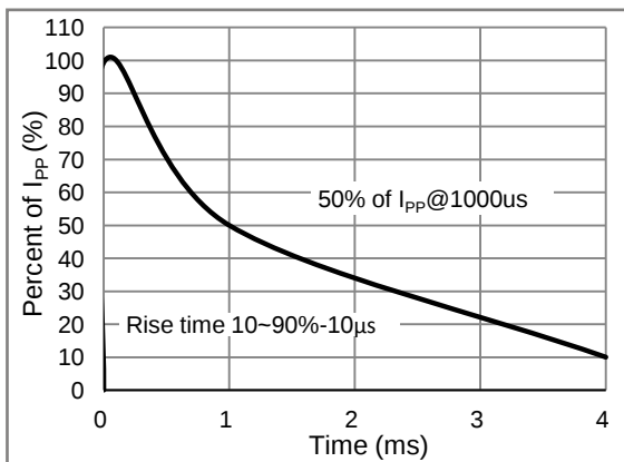
Fig.3 10/1000 \mu\text{s} Pulse Waveform
