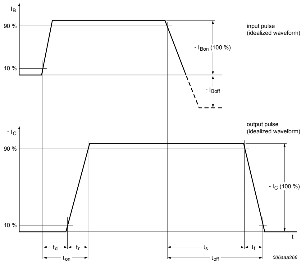
Fig. 28. TR2 (PNP): BISS transistor switching time definition
