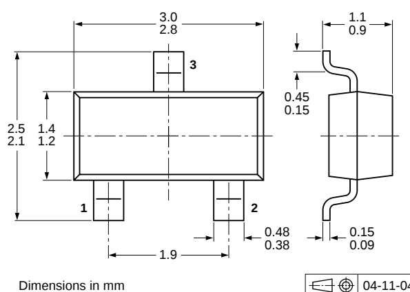
Fig 25. Package outline PDTB1xxxT series (SOT23/TO-236AB)
