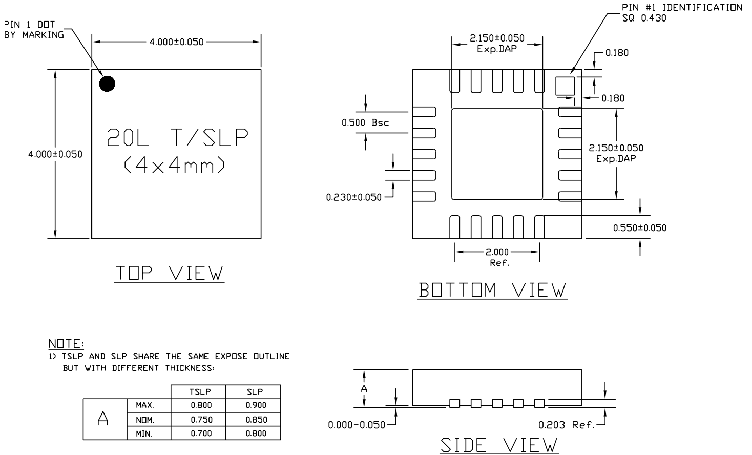
Figure 20. Package Drawing
