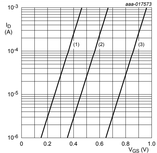
T_j = 25 \text{ }^\circ\text{C} ; V_{DS} = 5 \text{ V} (1) minimum values (2) typical values (3) maximum values
