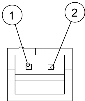
Connector A Manufacturer - JST Part #s S2B-PH-K-S Plug entry view
