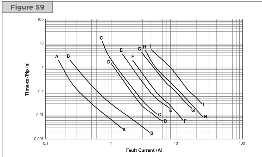
Figures S6-S15 — Typical Time-to-Trip Curves at 20°C
