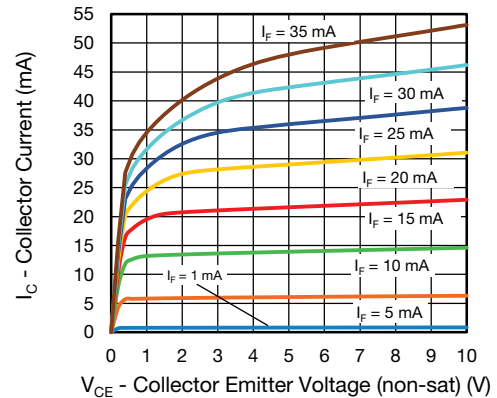
Fig. 2 - Collector Current vs. Collector Emitter Voltage (NS)
