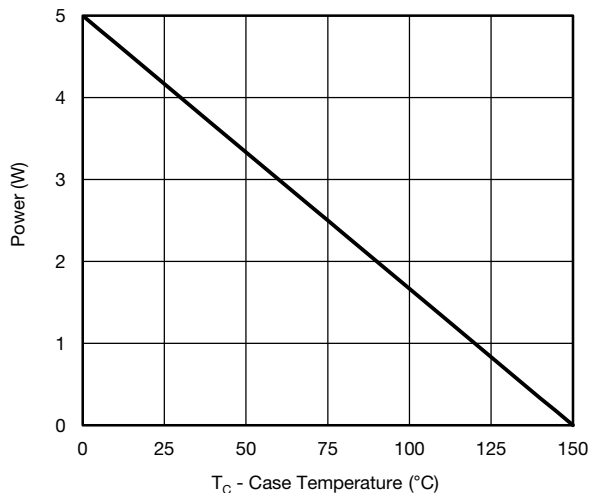
Power, Junction-to-Case
