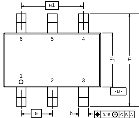
6-LEAD TSOP
