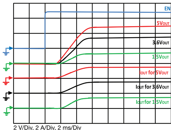
Fig. 19 - Typical Turn-On Delay, Rise Time C OUT = 0.1 μF, C IN = 4.7 μF, I OUT = 1.5 A
