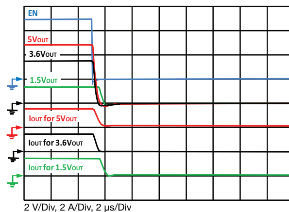
Fig. 20 - Typical Fall Time C OUT = 0.1 μF, C IN = 4.7 μF, I OUT = 1.5 A
