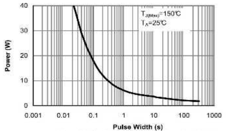
Figure 10: Single Pulse Power Rating Junction-to-Ambient (Note E)
