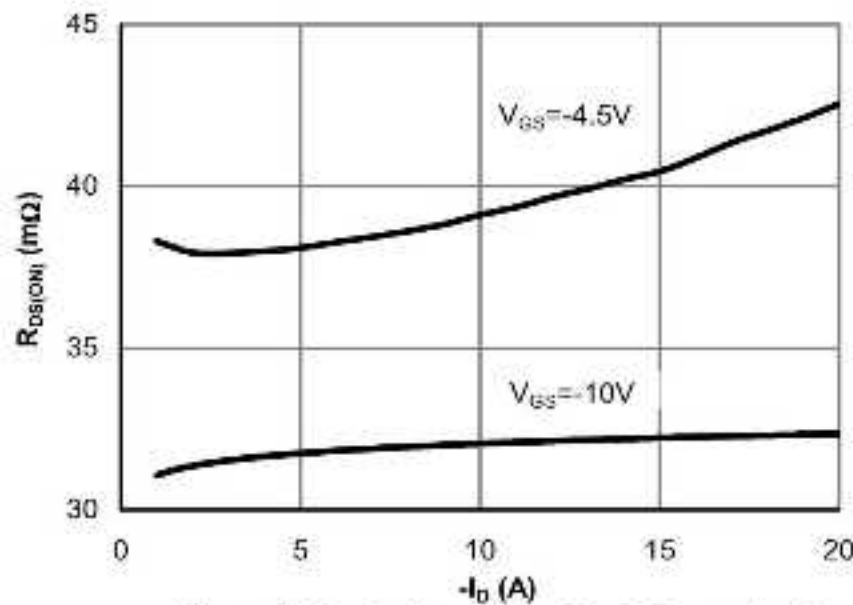
Figure 3: On-Resistance vs. Drain Current and Gate Voltage
