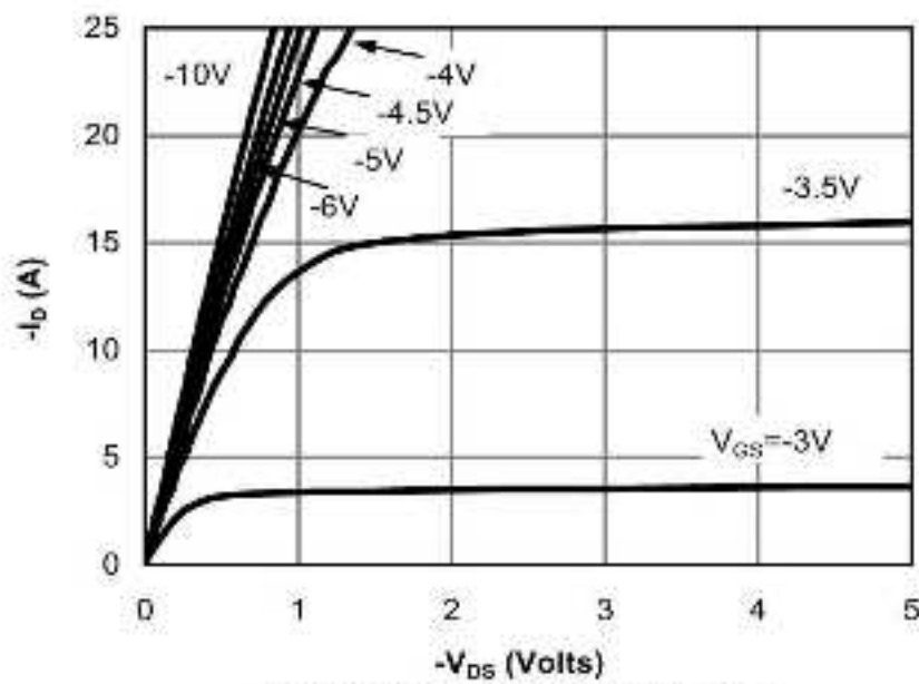
Fig 1: On-Region Characteristics
