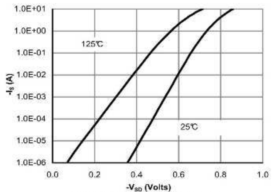
Figure 6: Body-Diode Characteristics
