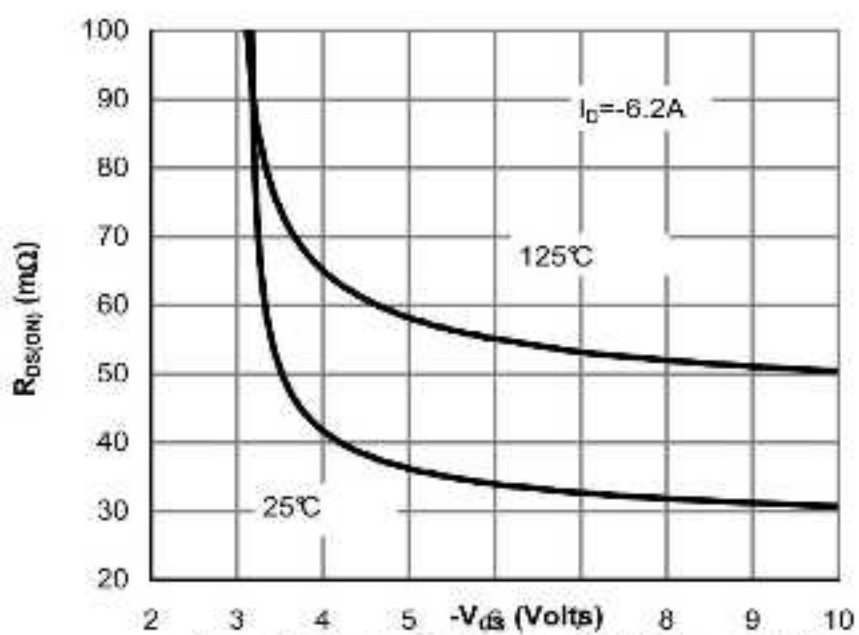
Figure 5: On-Resistance vs. Gate-Source Voltage
