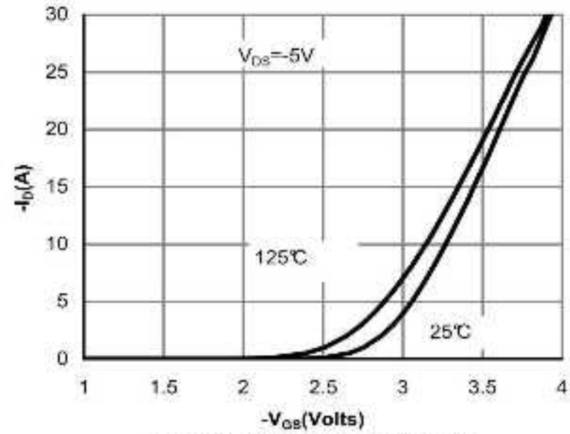
Figure 2: Transfer Characteristics
