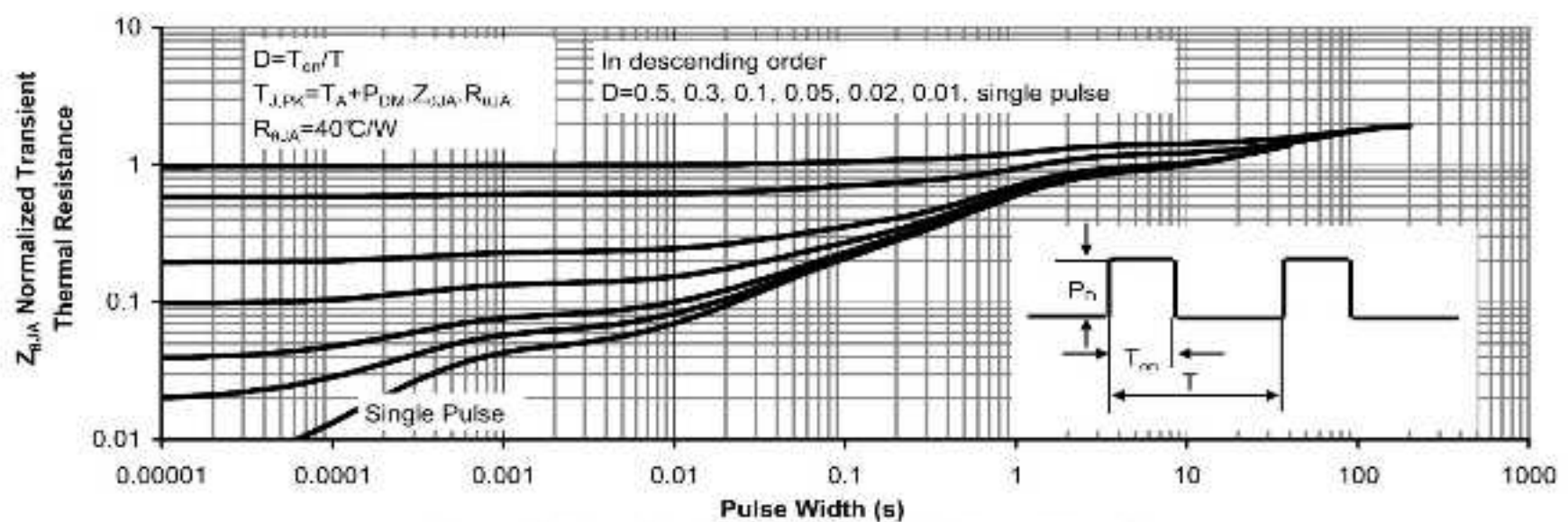
Figure 11: Normalized Maximum Transient Thermal Impedance
