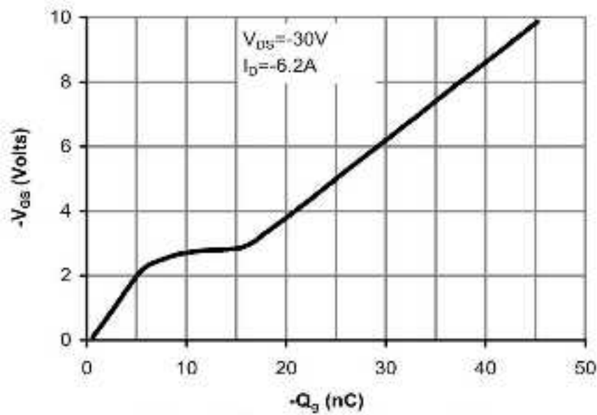
Figure 7: Gate-Charge Characteristics
