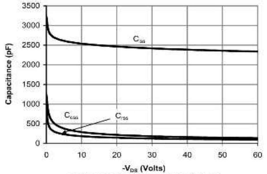
Figure 8: Capacitance Characteristics
