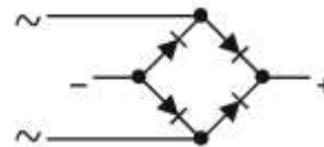
Equivalent Circuit
