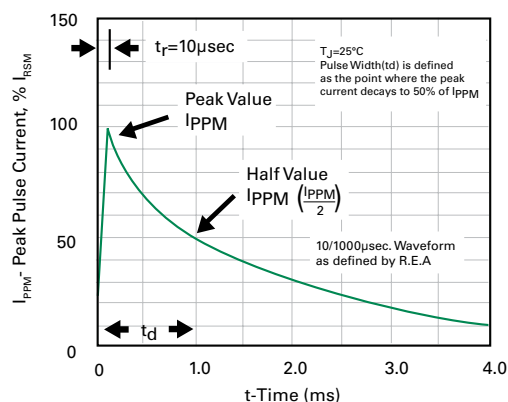
Figure 4 - Pulse Waveform
