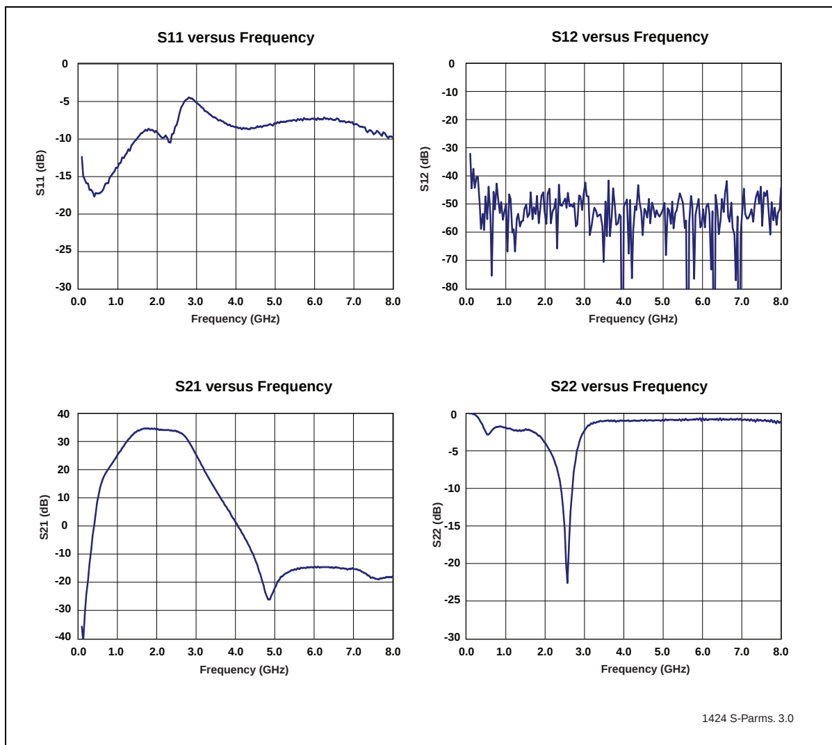
Figure 5: S-Parameters
