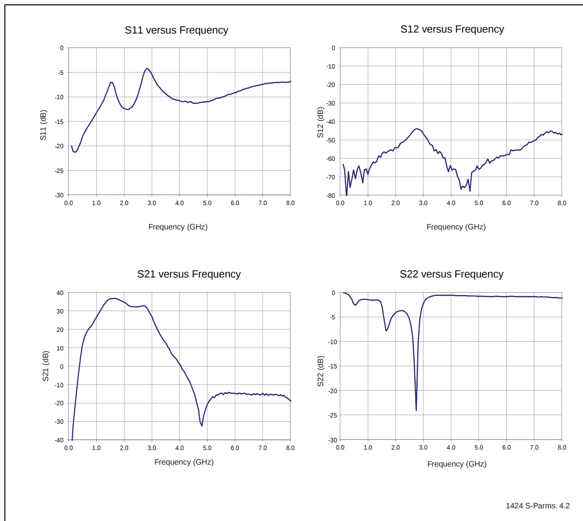
Figure 20: S-Parameters
