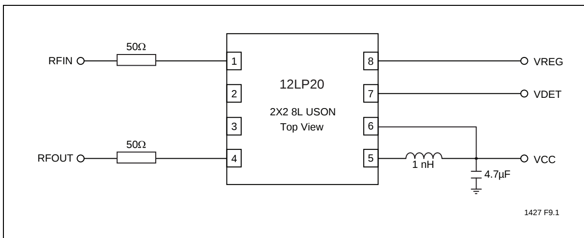
Figure 9: Typical Schematic for High-Efficiency 802.11b/g Applications
