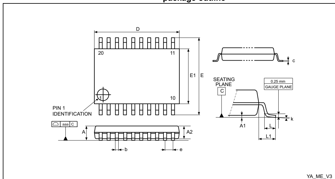
Figure 28. TSSOP20 – 20-lead thin shrink small outline, 6.5 x 4.4 mm, 0.65 mm pitch, package outline
