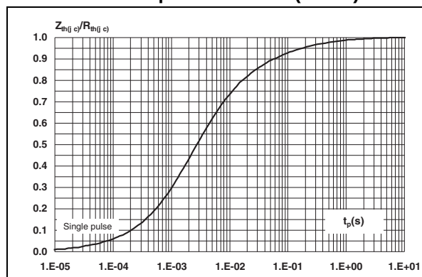
Figure 7. Relative variation of thermal impedance junction to case versus pulse duration (DPAK)
