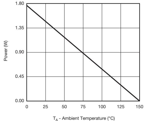
Power, Junction-to-Ambient
