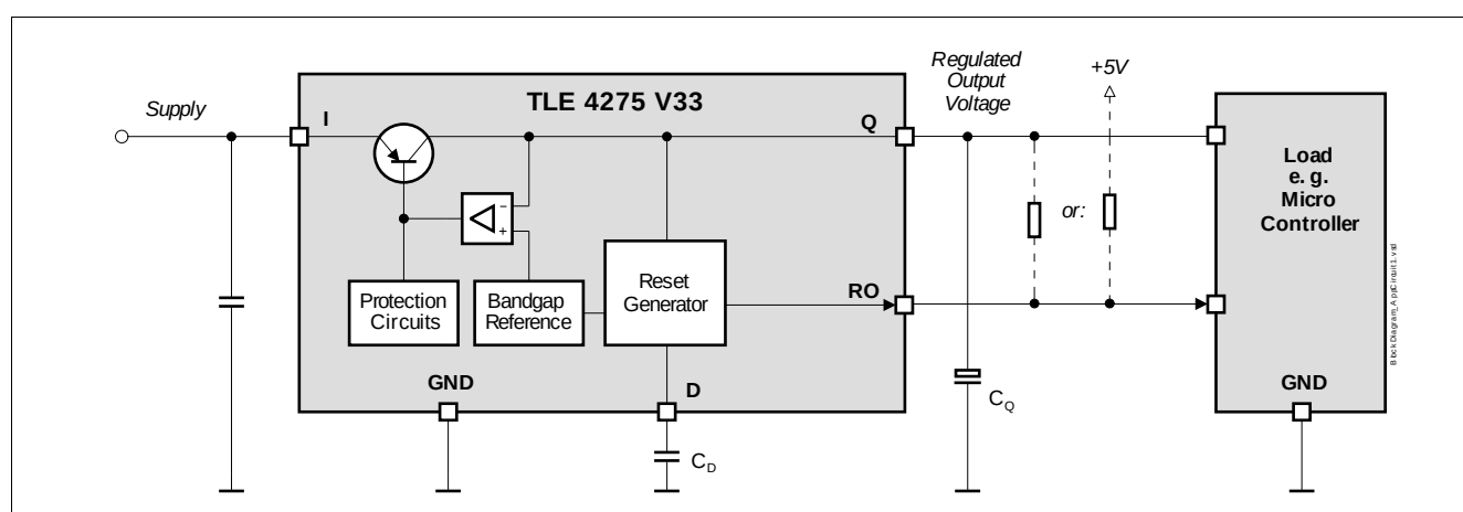
Figure 1 Simplified Block Diagram and Typical Application
