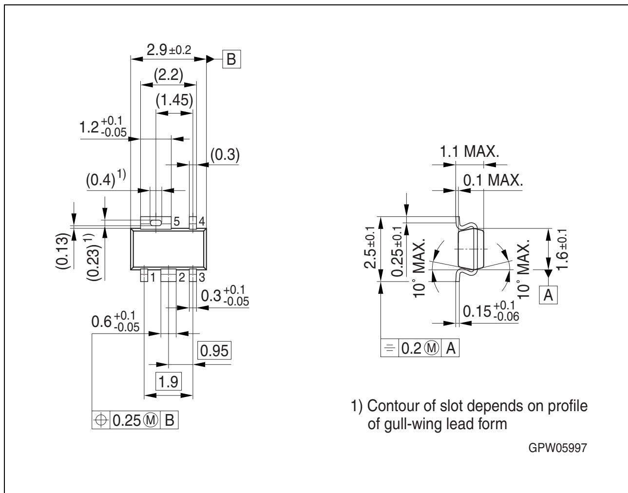
Figure 4 Outline PG-SCT-595-5
