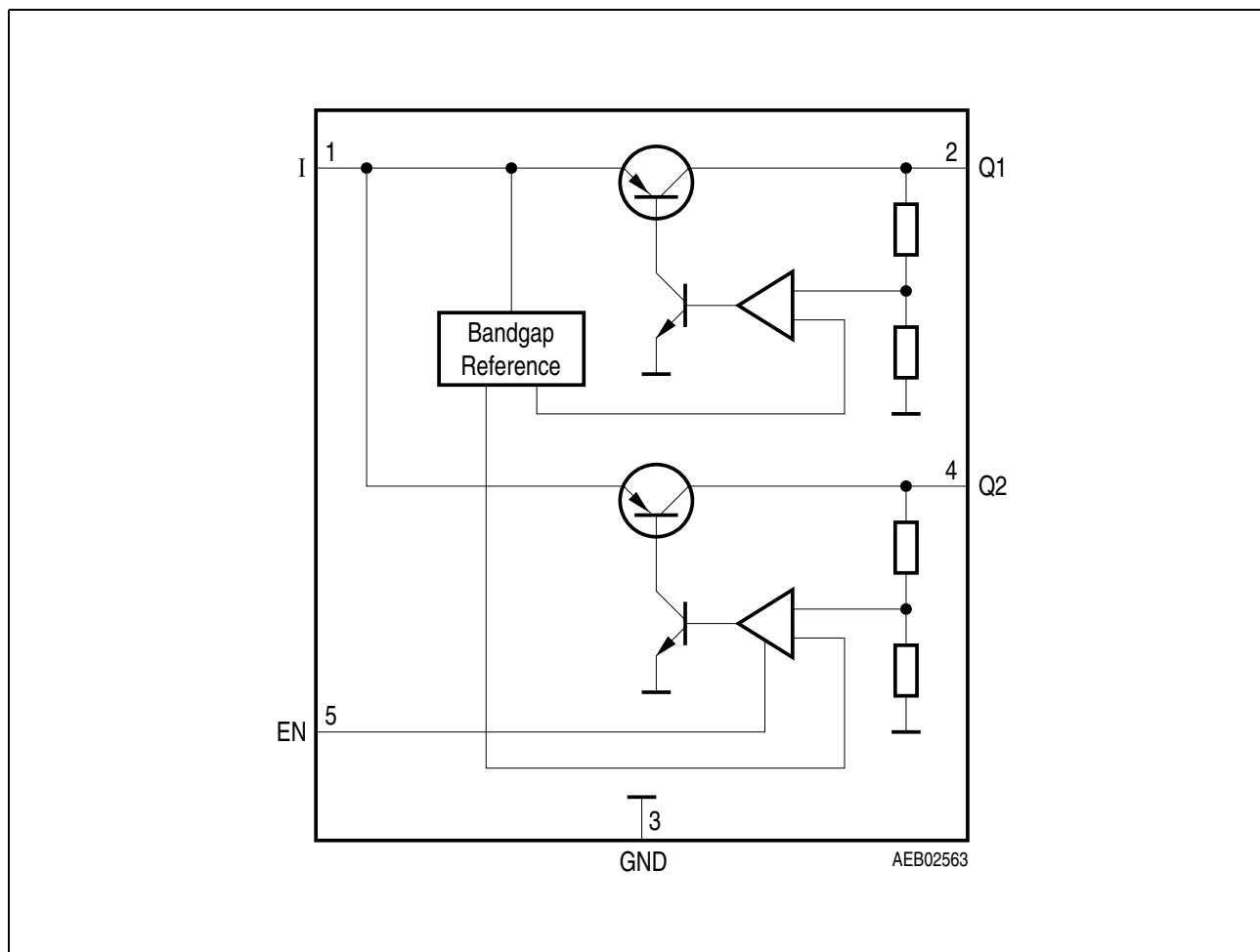
Figure 2 Block Diagram
