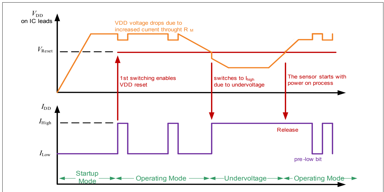
Figure 6 Undervoltage Behavior
