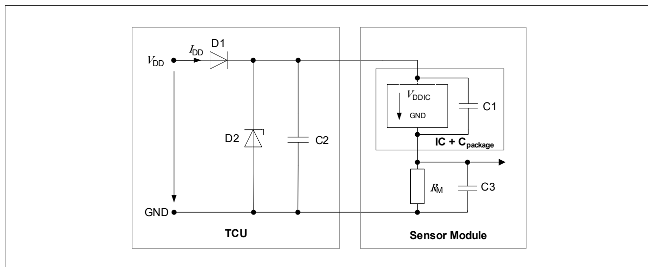
Figure 10 Application circuit
