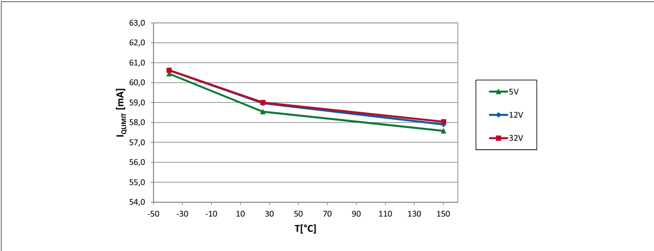
Figure 23 Output current limit of the TLE4964-1K over temperature
