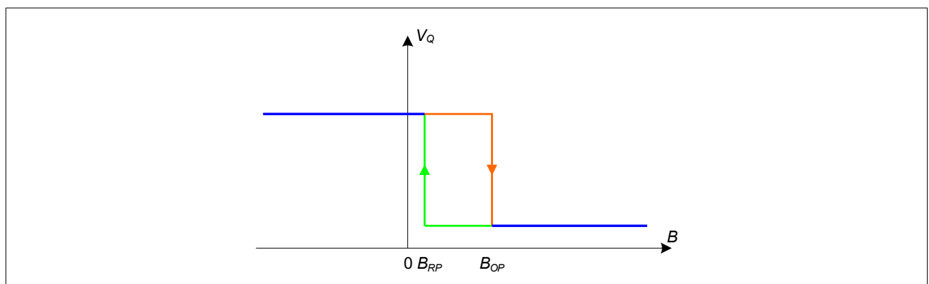
Figure 5 Output signal TLE4964-1K
