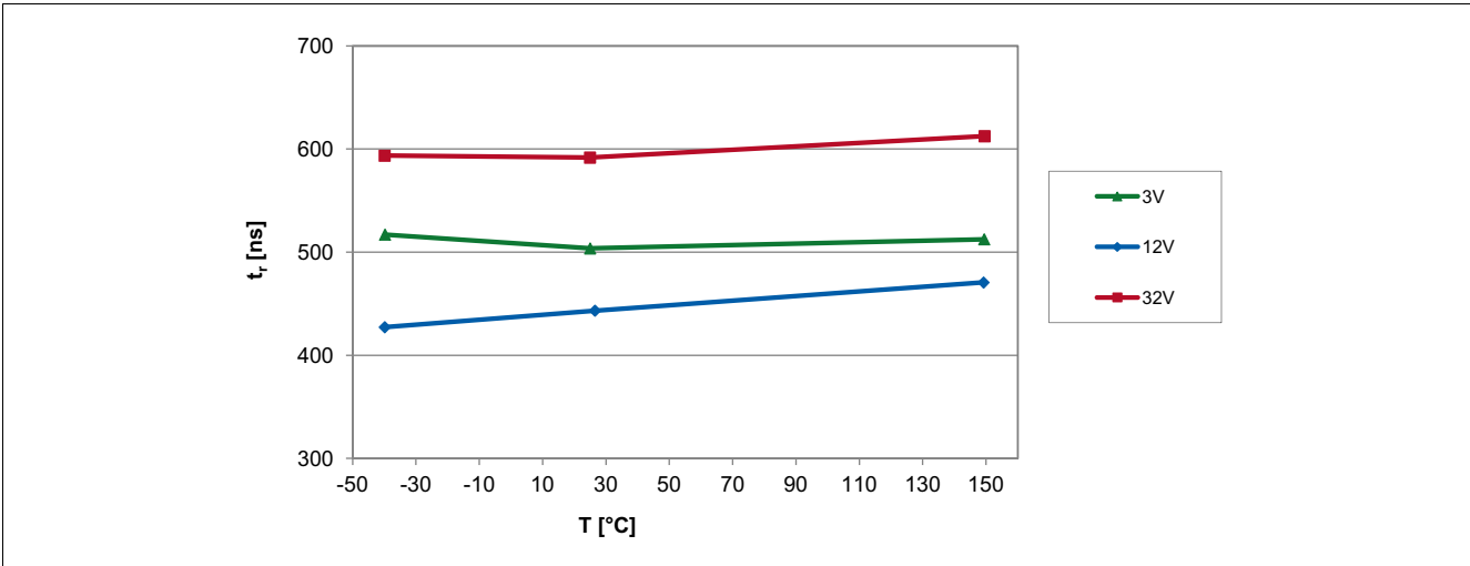
Figure 27 Output rise time of the TLE4964-1K over temperature
