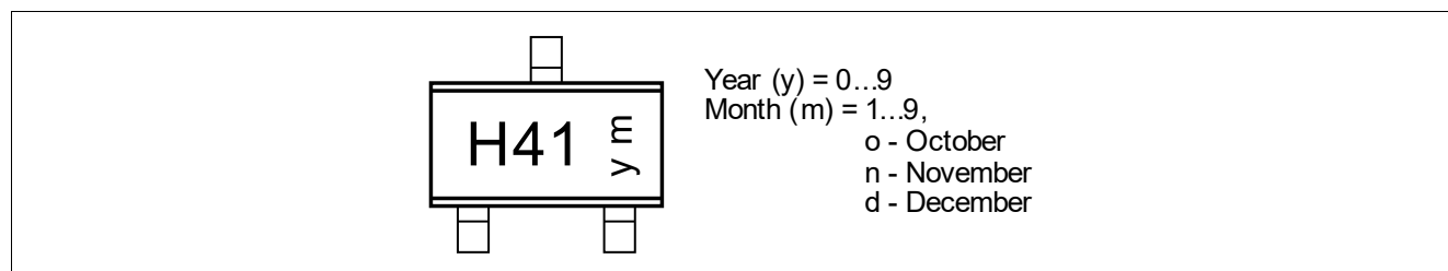
Figure 15 Marking of TLE4964-1K
