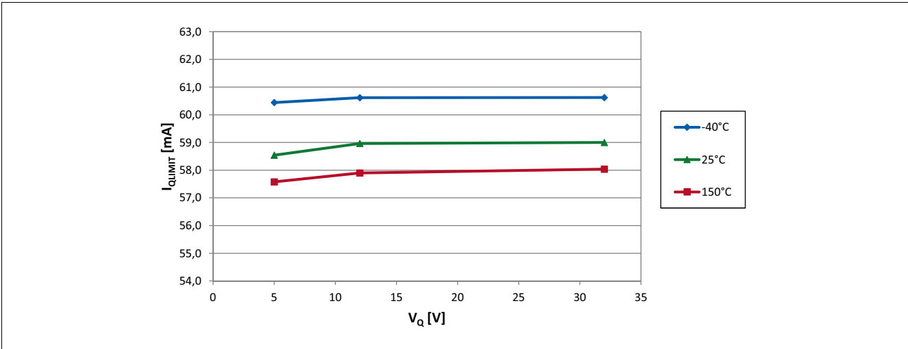
Figure 24 Output current limit of the TLE4964-1K over applied pull-up voltage
