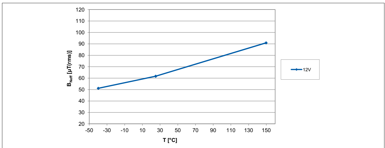
Figure 32 Effective noise of the TLE4964-1K thresholds over temperature
