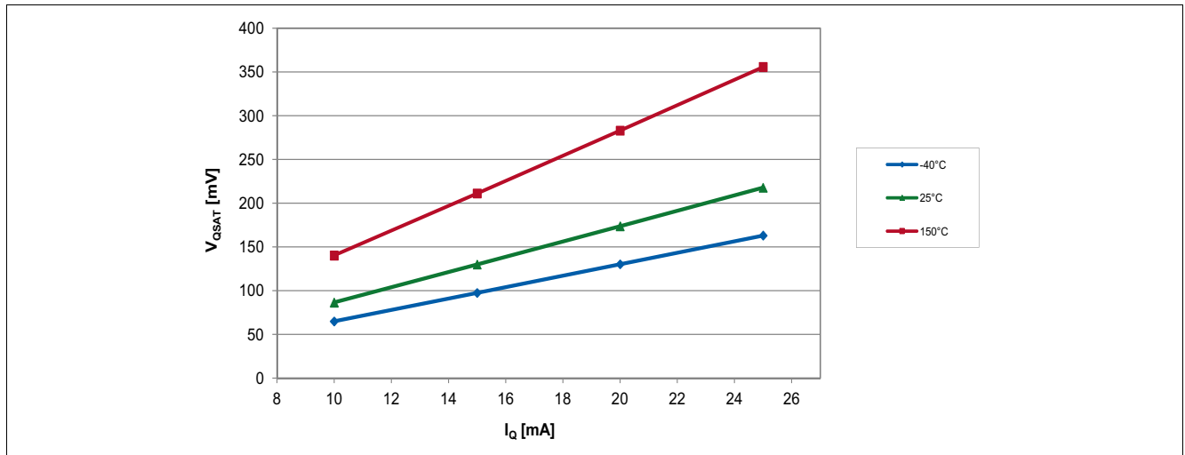
Figure 31 Saturation voltage of the TLE4964-1K over output current
