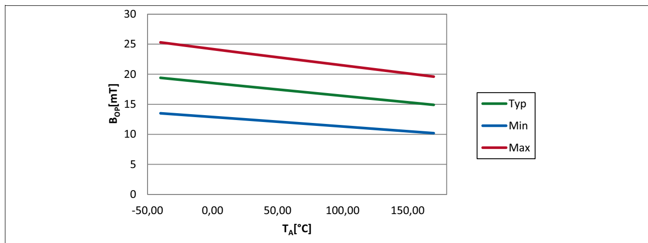
Figure 16 Operating point ( B_{OP} ) of the TLE4964-1K over temperature
