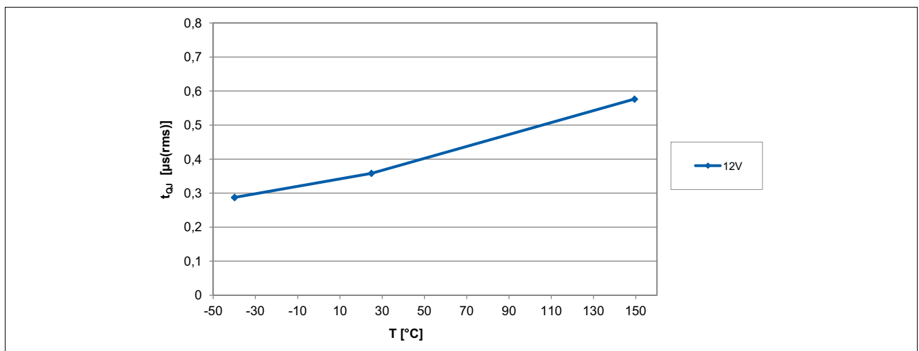
Figure 33 Output signal jitter of the TLE4964-1K over temperature
