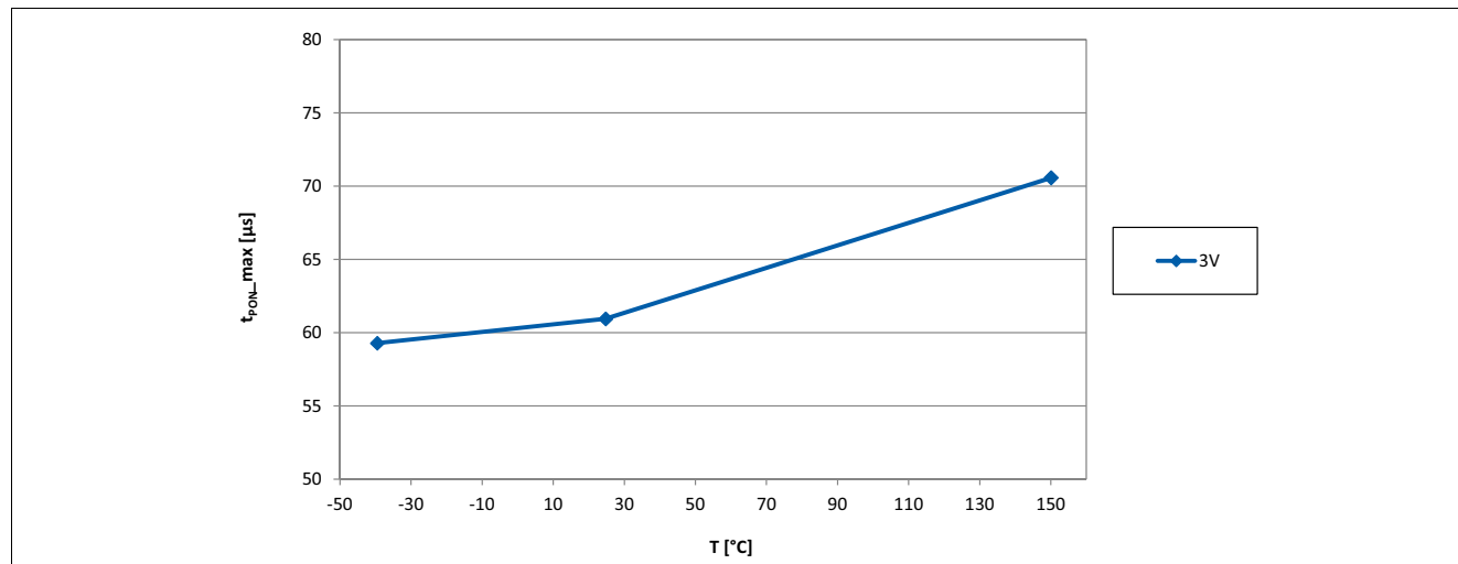
Figure 19 Power on time t_{PON} of the TLE4964-1K over temperature
