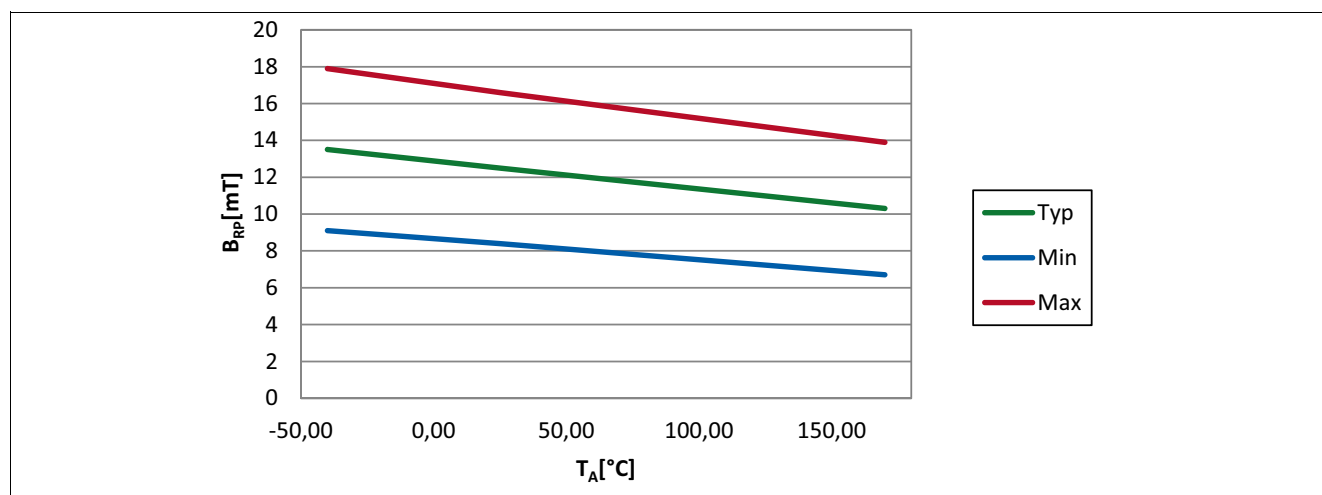
Figure 17 Release point ( B_{RP} ) of the TLE4964-1K over temperature
