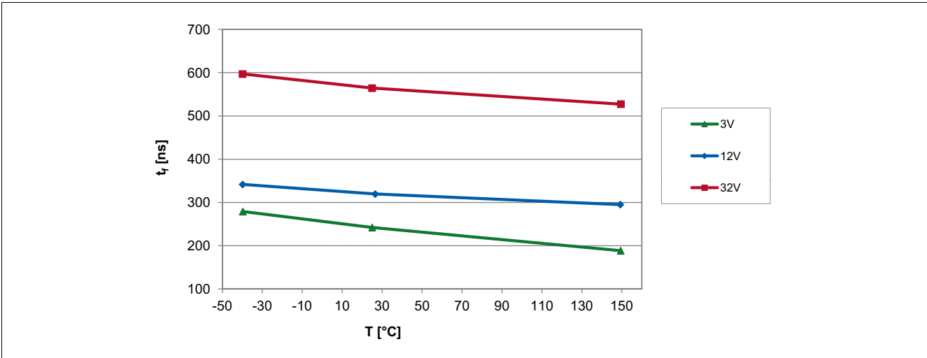
Figure 25 Output fall time of the TLE4964-1K over temperature
