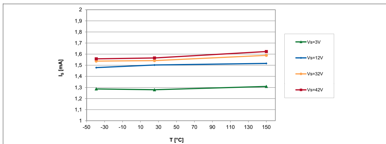
Figure 21 Supply current of the TLE4964-1K over temperature
