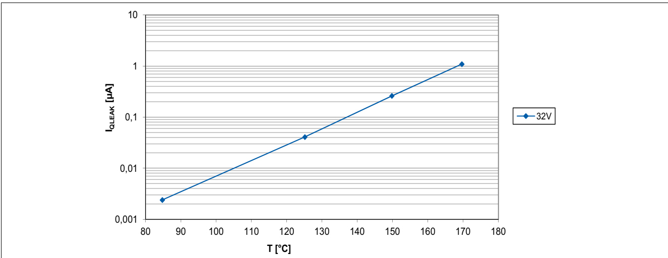
Figure 29 Output leakage current of the TLE4964-1K over temperature
