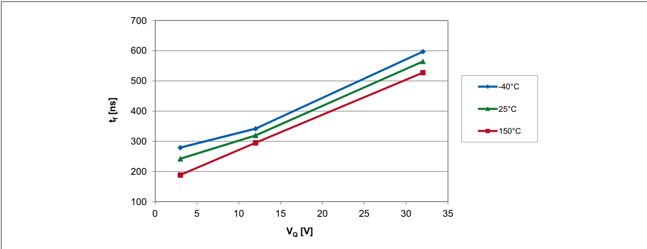
Figure 26 Output fall time of the TLE4964-1K over applied pull-up voltage
