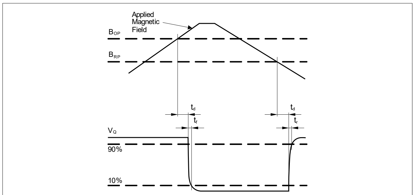
Figure 4 Timing diagram TLE4964-1K
