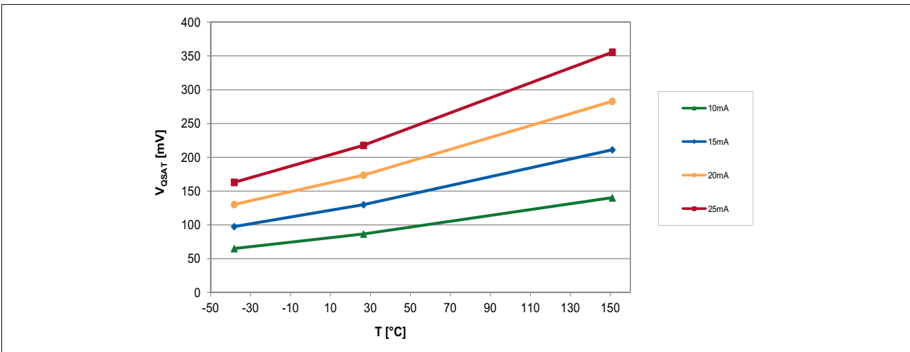
Figure 30 Saturation voltage of the TLE4964-1K over temperature
