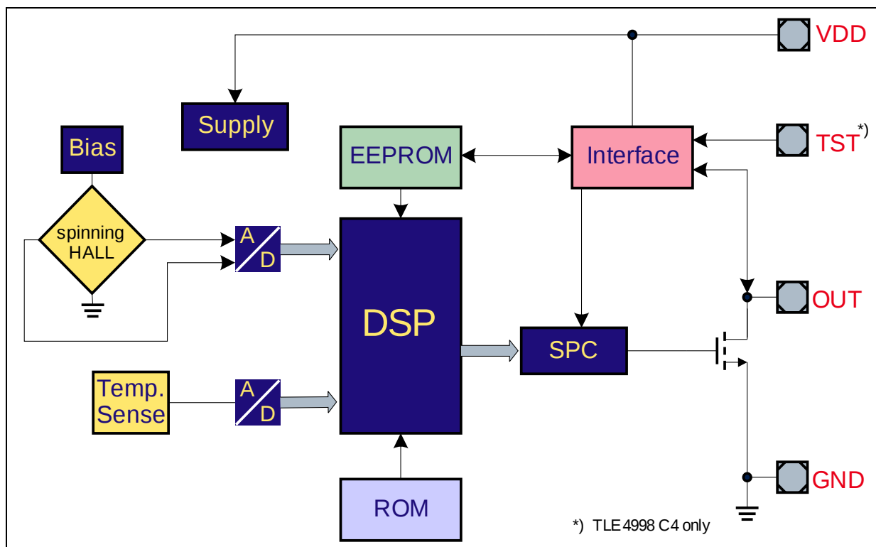
Figure 3 Block diagramm
