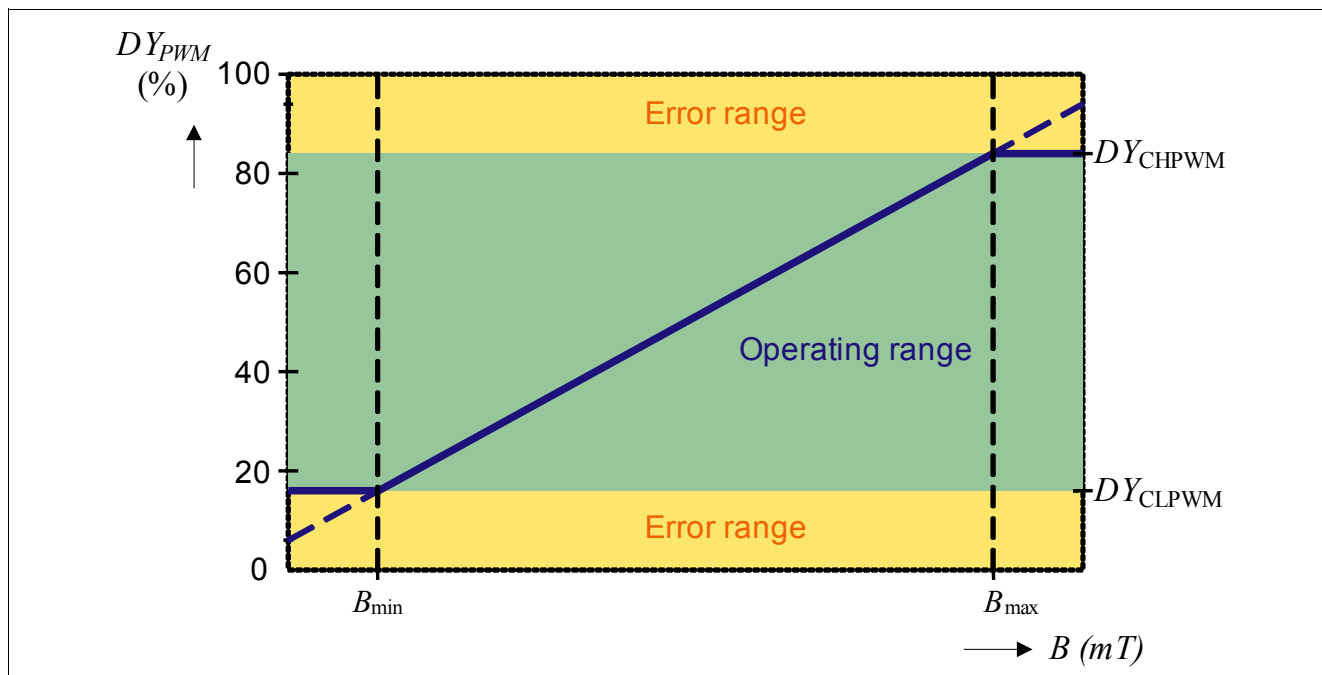
Figure 7-1 Clamping Example
