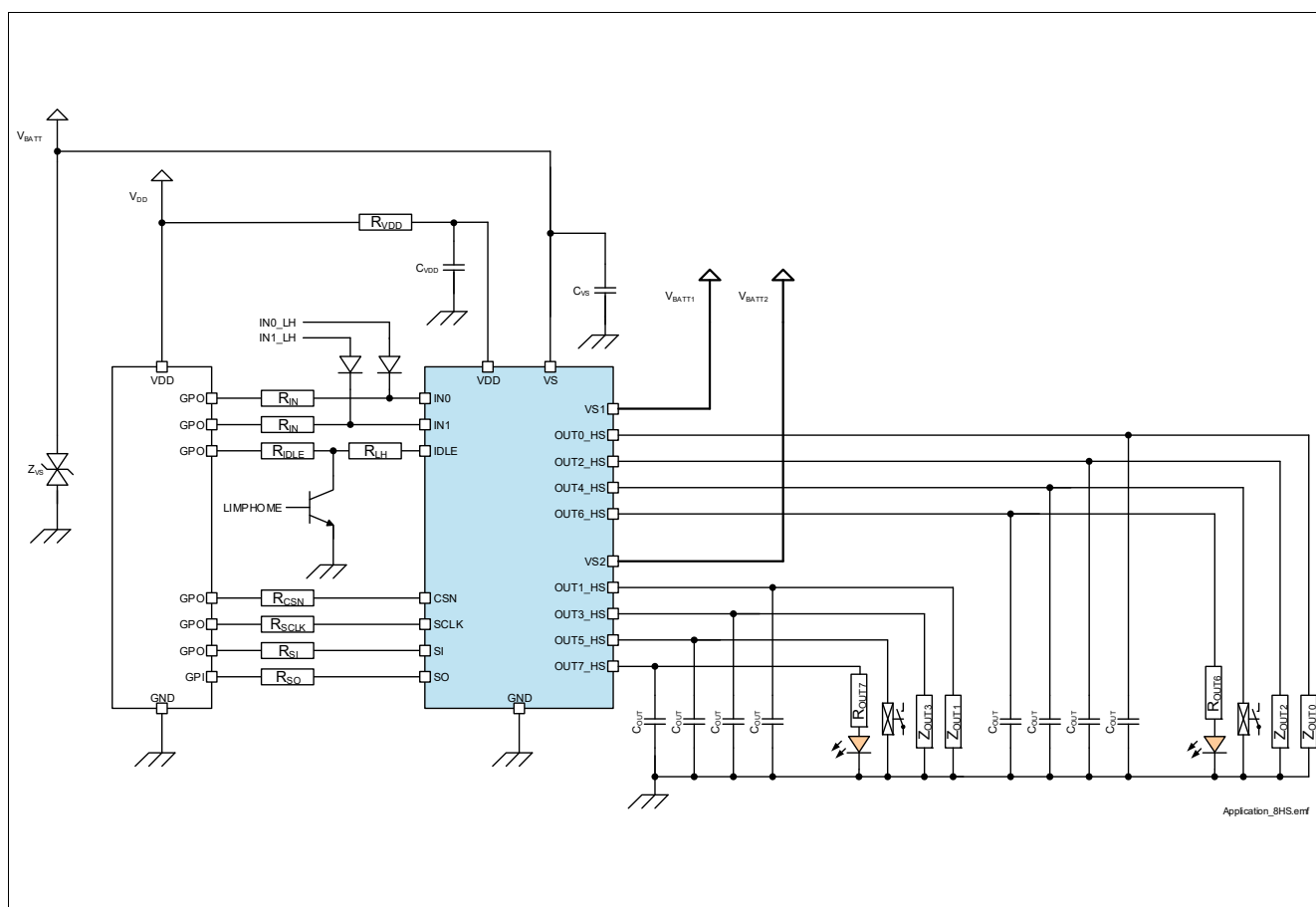
Figure 1 TLE75080-ESH Application Diagram
