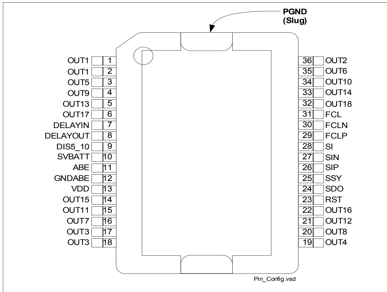
Figure 3 Pin Assignment
