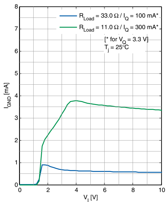
GND Pin Current I_{\text{GND}} versus Input Voltage V_{\text{I}} (TLS203B0EJV33)
