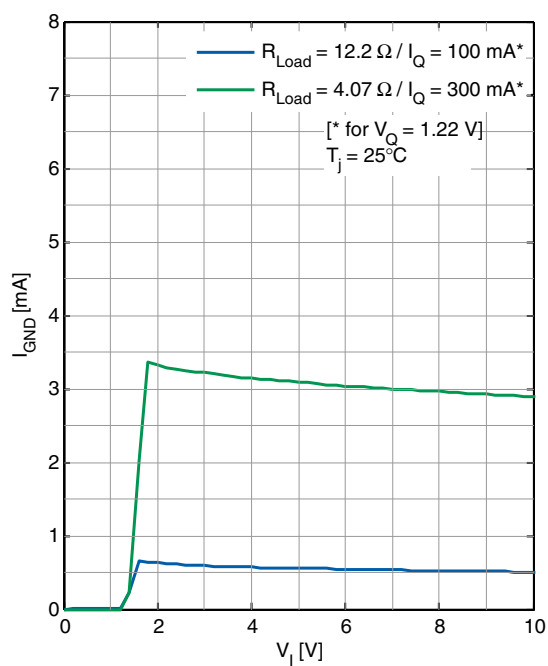
GND Pin Current I_{\text{GND}} versus Input Voltage V_{\text{I}} (TLS203B0EJV)
