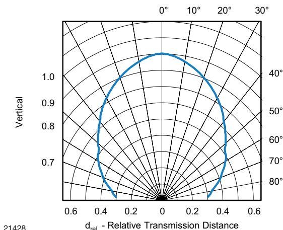
Fig. 12 - Vertical Directivity
