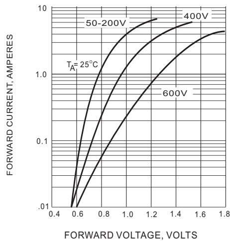
Fig.3 FORWARD CHARACTERISTICS
