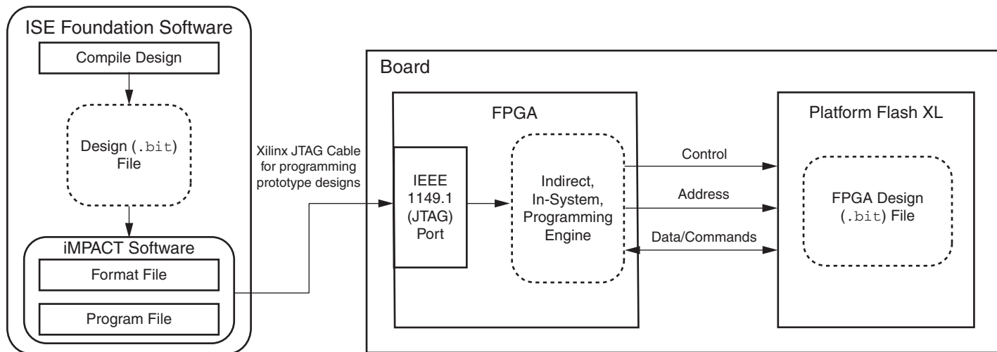
Figure 7: Integrated FPGA Design and In-System Programming Solution for Platform Flash XL
