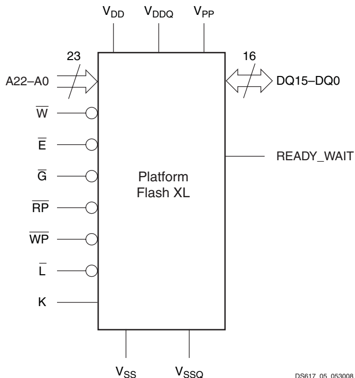
Figure 5: Logic Diagram
