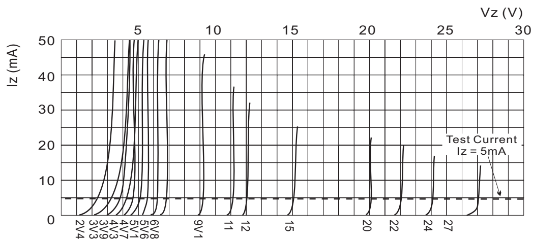
Fig.2 BREAKDOWN CHARACTERISTICS
